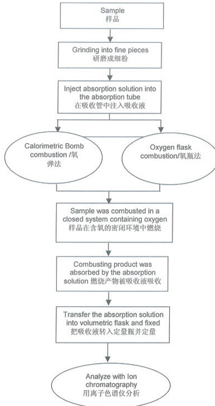
Test Procedures Flow Chart for the determination of Halogen 卤素测试流程图
