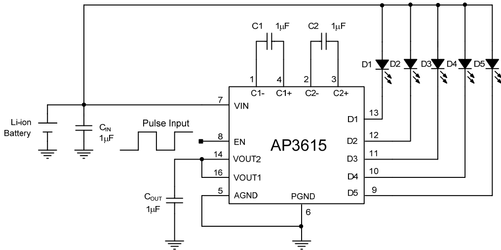
5 WLEDs
