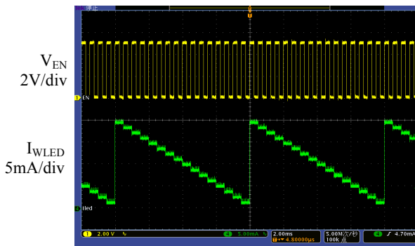
Time (2ms/div)
